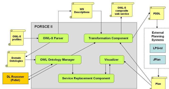
Figure 1 PORSCE II architecture.
