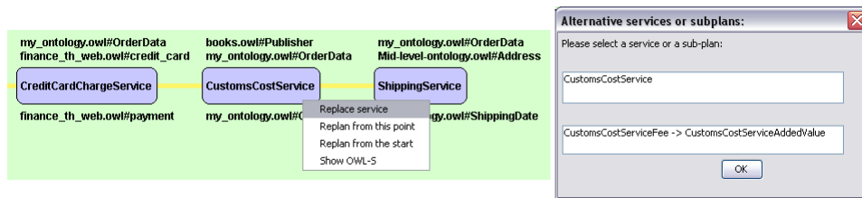
Figure 11 Service Replacement Interface.
