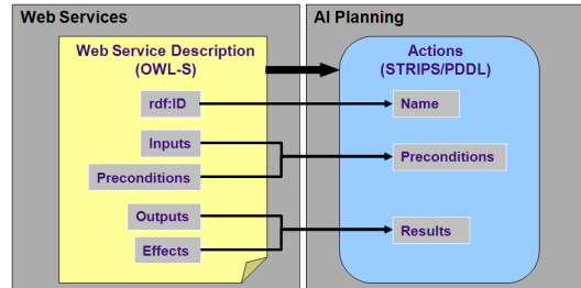
Figure 2 Web services to planning domain mapping.
