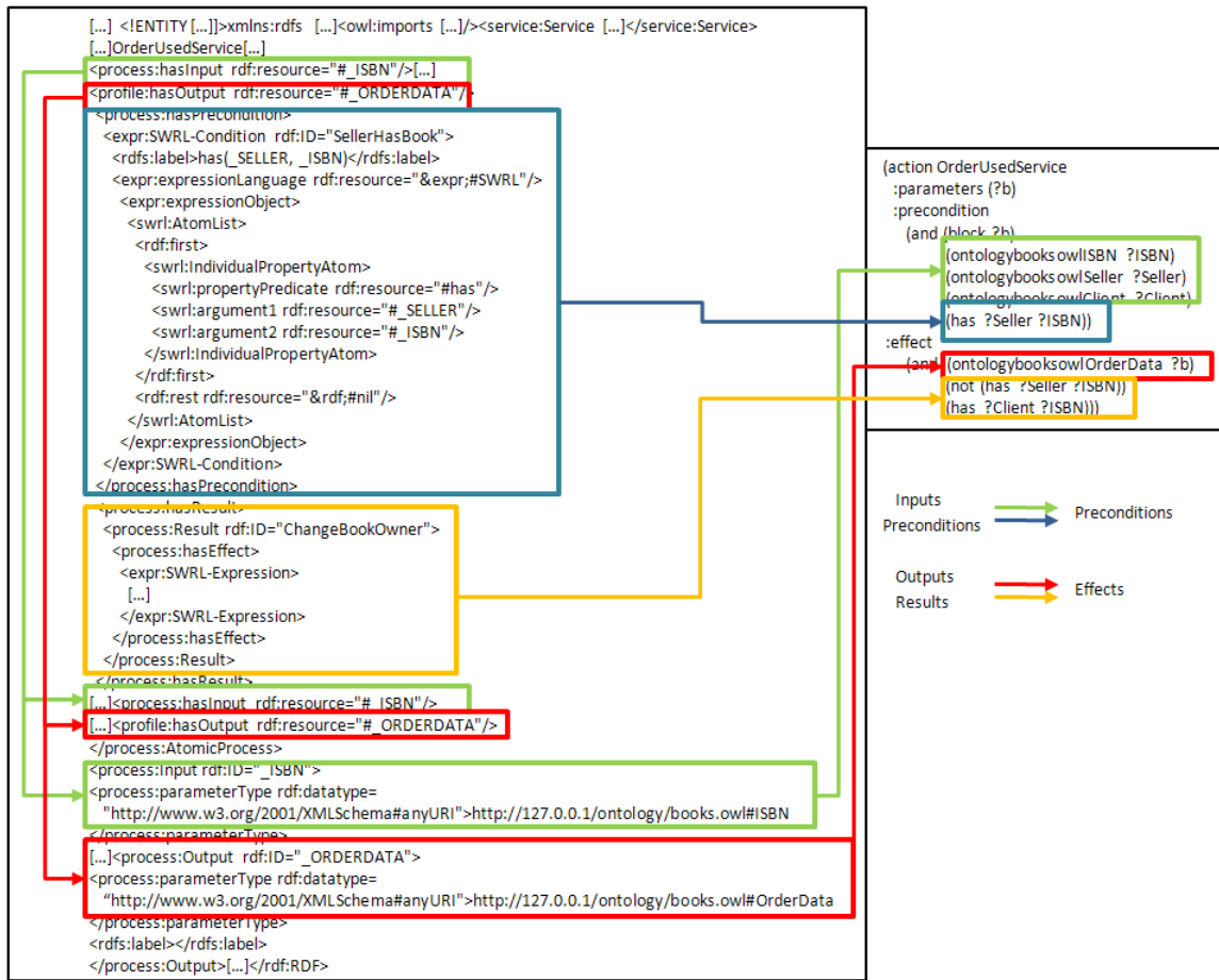
Figure 3 OWL-S to PDDL translation example.
