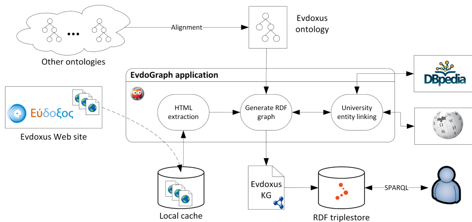
Figure 1. Knowledge Graph generation workflow.
