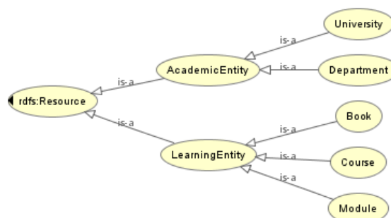
Figure 3. Class hierarchy of the Evdoxus ontology.
