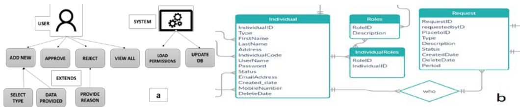
Figure 2: (a) Functional requirements of isU system regarding new request – (b) Part of the ER diagram
