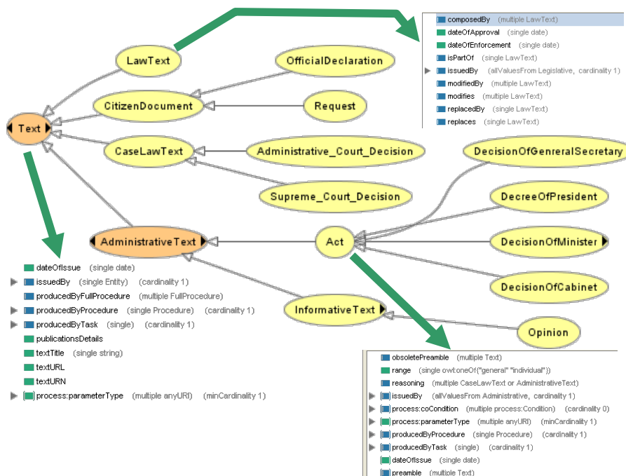
Figure 4. The textual aspect of the ontology of public administration procedures.
