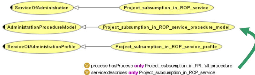
Figure 11. Service, service profile and service model of the case study.
