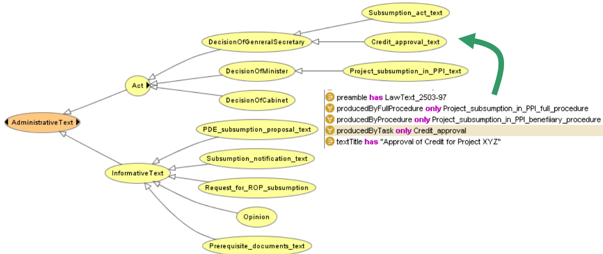
Figure 12. Administrative Documents of the case study.
