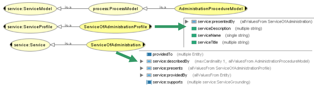
Figure 6. Specializations of OWL-S Service, Service Profile and Service Model
