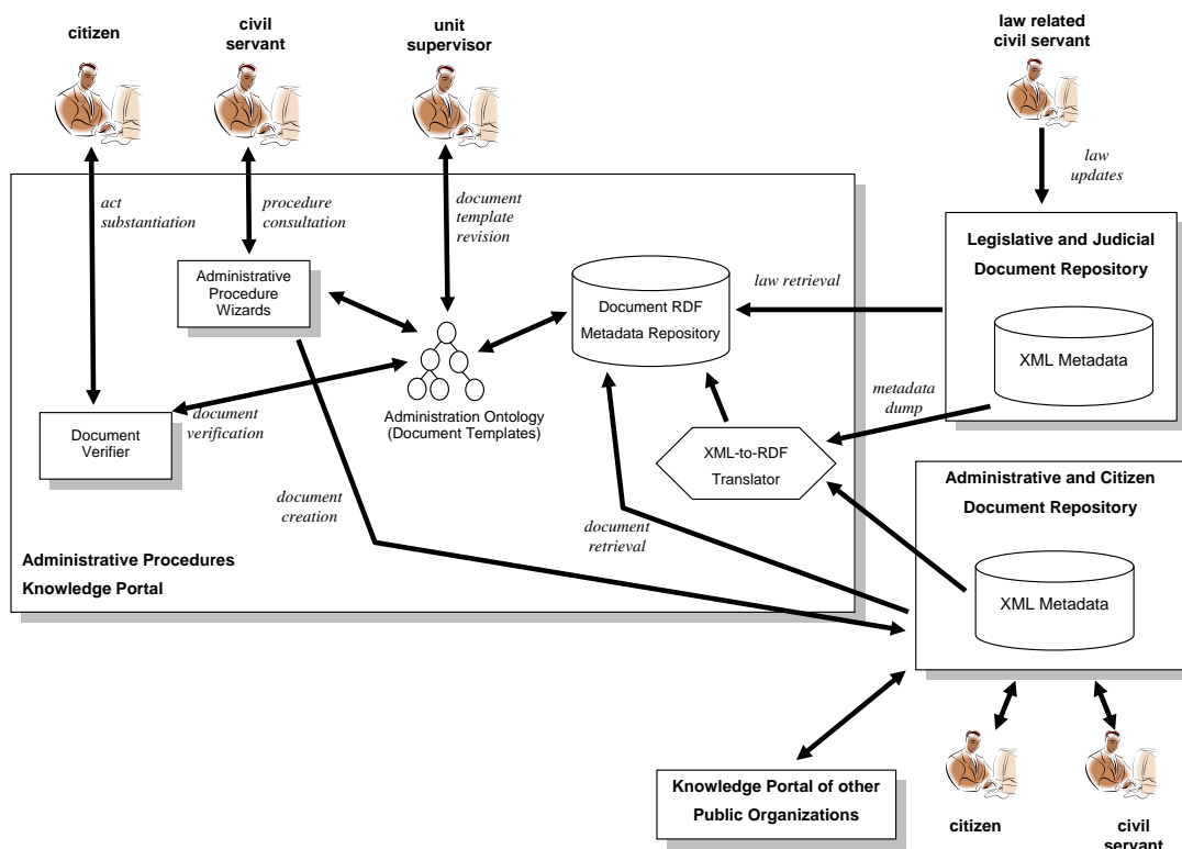
Figure 2. Architecture of the Administrative Procedures Knowledge Portal
