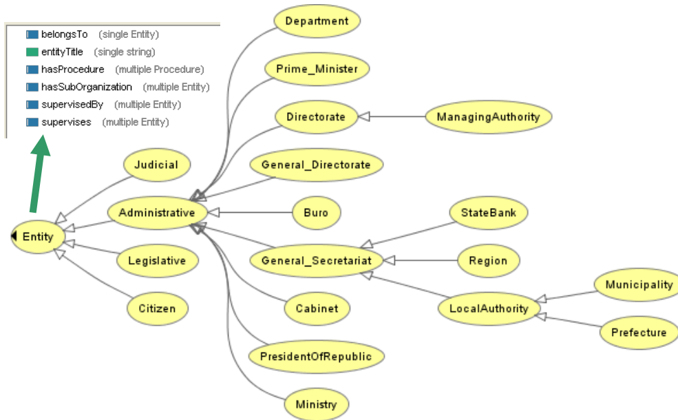
Figure 3. The structural aspect of the ontology of public administration procedures.
