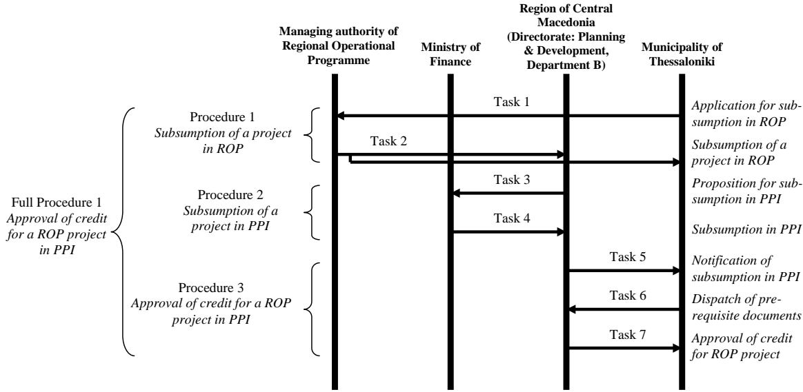
Figure 8. Example of an administrative service (full procedure) and its environment.
