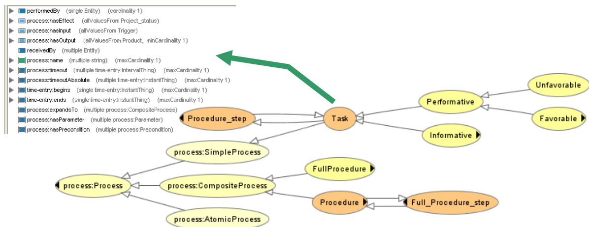
Figure 5. The public administration procedure ontology as an extension of OWL-S
