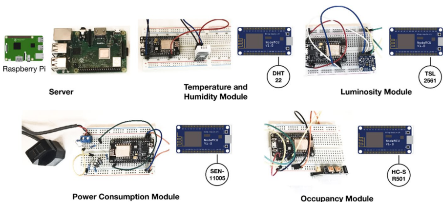
Fig. 3 Custom sensors by Alsalemi et al. (2019a)
